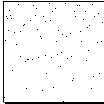
Random B
