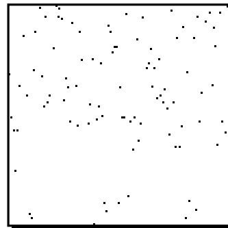
Random F
