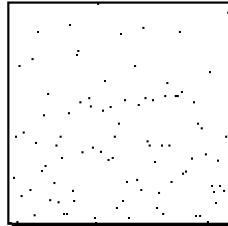
Random D
