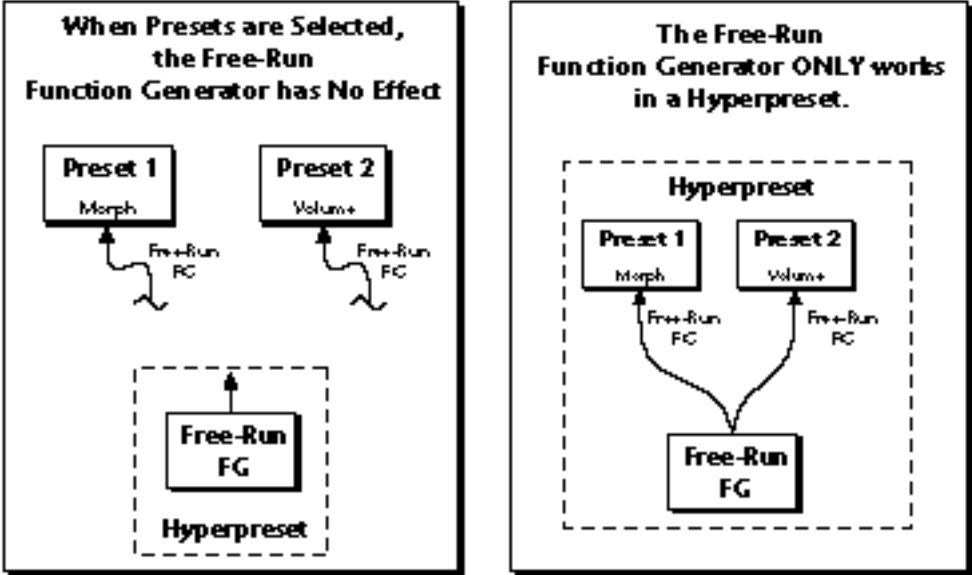
The Free-Run Function Generator only works in a Hyperpreset, even though the modulation routing is made in the preset.
